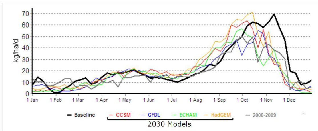
Figure above - Actual modelled output – 4 GCM's, Lismore Victoria – current and 2030
